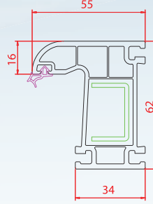
Dar Kasa
